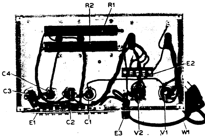
FIG. 5—Bottom view of power supply.
