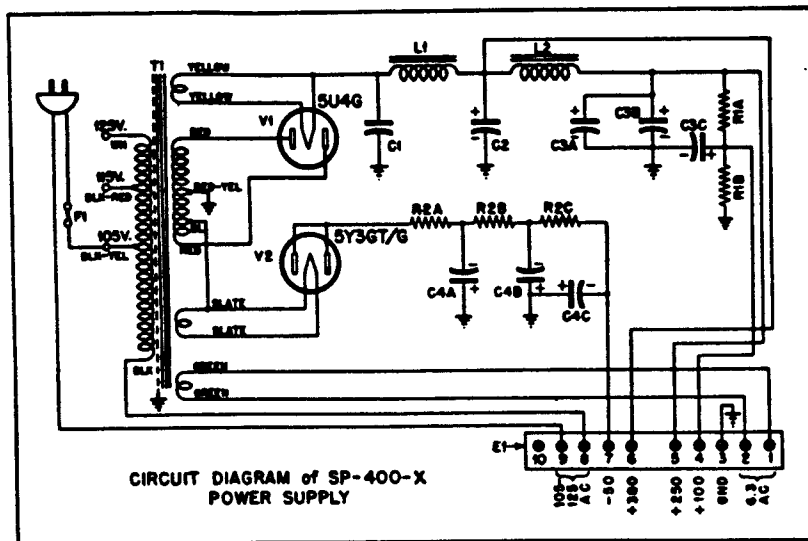
FIG. 10— Power supply diagram.
