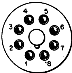
OCTAL BASE (BOTTOM VIEW)
