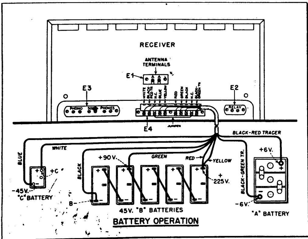
FIG. 4—Connections for power cable—battery operation.
