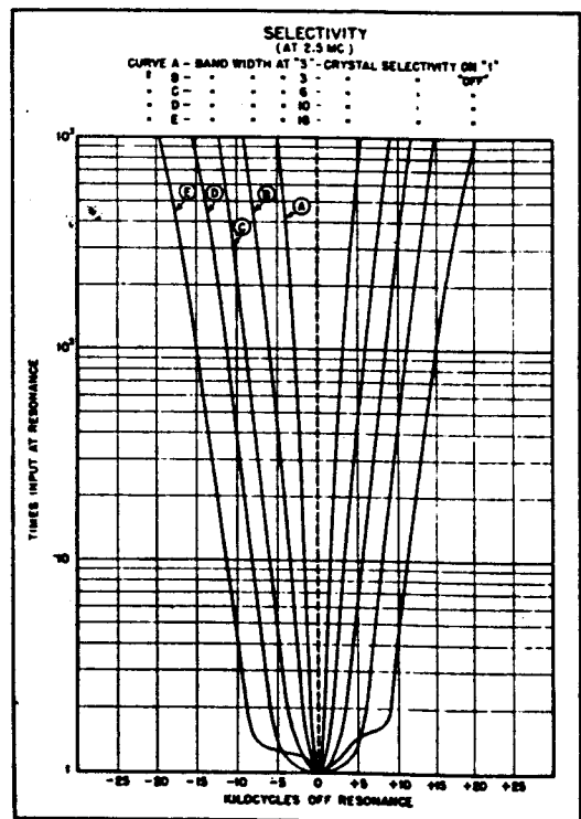
FIG. 8—Selectivity curves.
