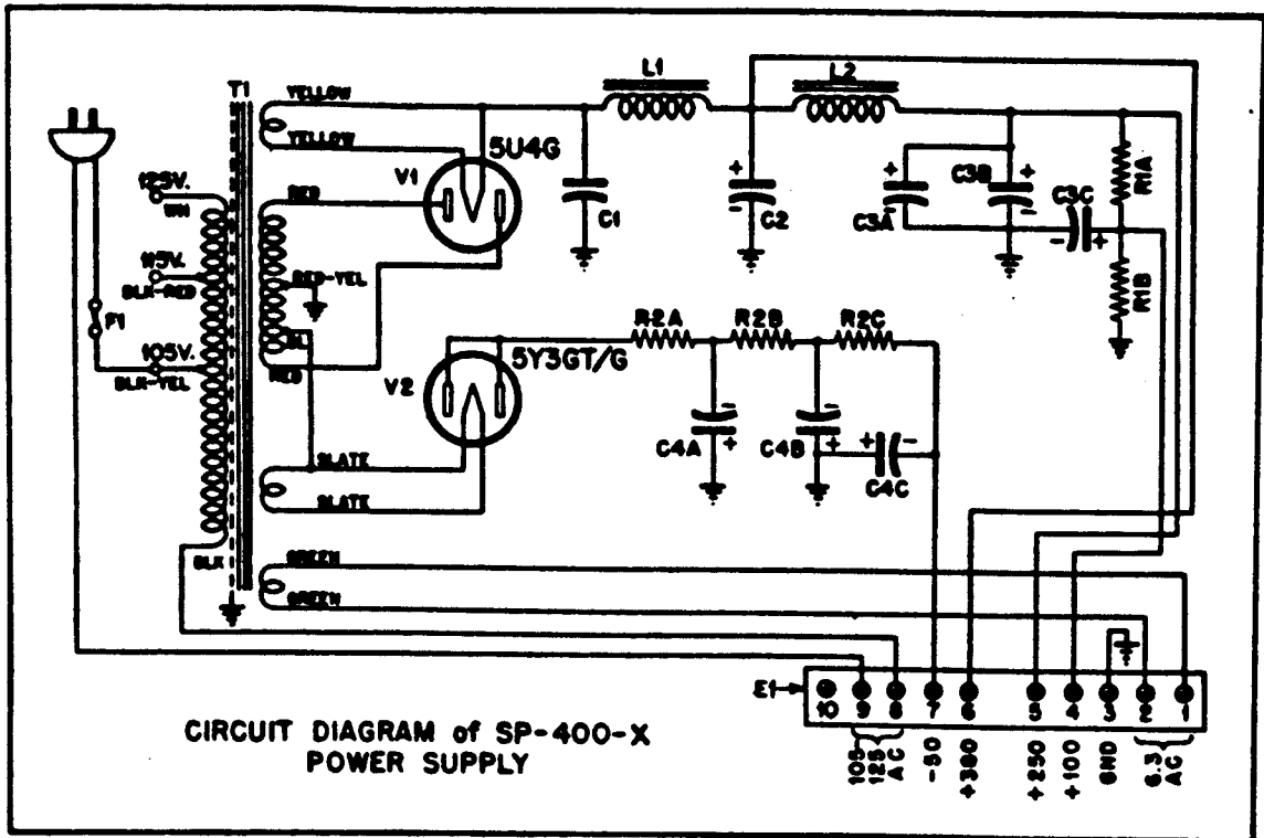
FIG. 10— Power supply diagram.
