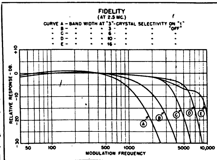
FIG. 9—Audio fidelity curves.
