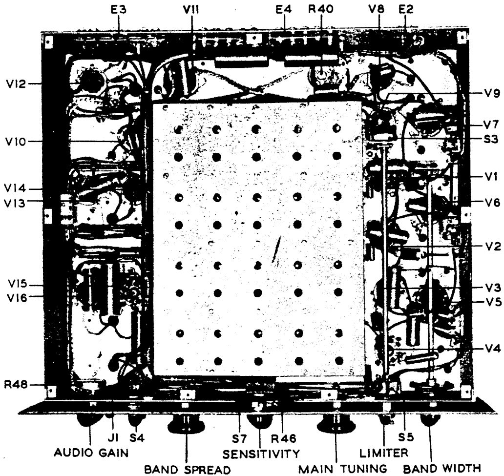
FIG. 12—Bottom view of chassis.
